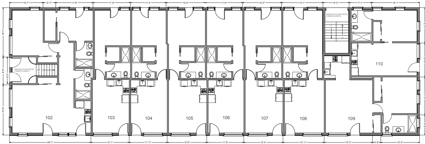
BOGART CONDOMINIUM - FIRST FLOOR (GROUND)
